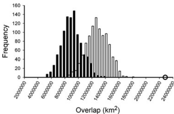
Figure 4 Randomization tests for overlap between important regions for terrestrial and freshwater biodiversity. Bars represent distribution from 1,000 spatial randomizations, both globally (black bars) and within each of the world’s 14 terrestrial biomes (white bars). Circle marks the observed overlap. In both cases, the observed overlap is greater than that generated by all 1,000 randomizations ( P < 0.001 ).
